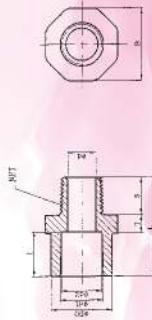
外牙接頭 (簡接頭) Male adapter
